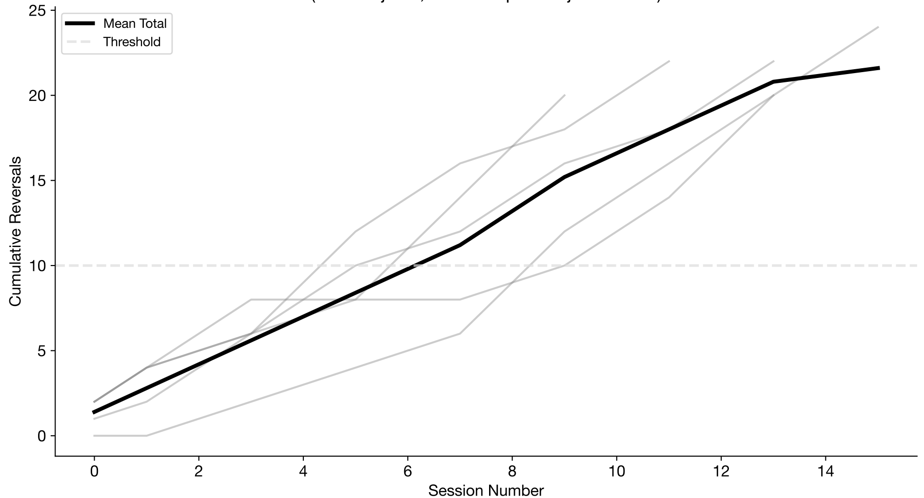
Cumulative Total Reversals Over Time (n=5 subjects; sessions per subject=10–16)
